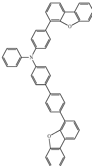
Chemical Formula 2-2
