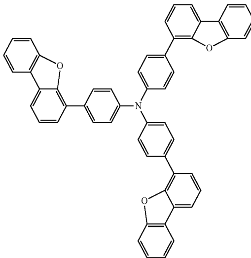
Chemical Formula 1-1
